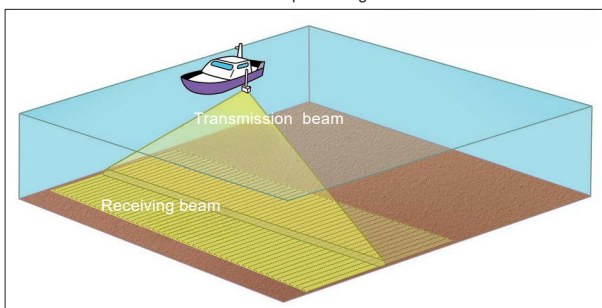
Conceptual Diagram of the Mills Cross Method
