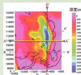
Gravity Structural Map of Basement Rock
